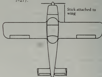
FIGURE 7-27. Checking blade track.
